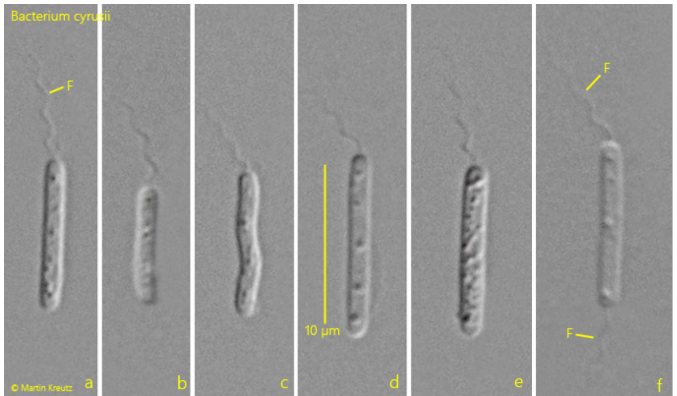
Fig. 2 a-f: Bacterium cyrusii . L = 6.8–11.8 µm. Some specimen in detail. The most specimens have one visible flagellum (F) but specimens with 2 visible flagella were also present (f). Obj. 100 X.
